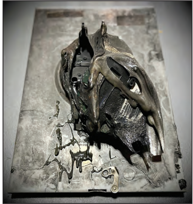
Image from Local 25 work, showing result of failure of an AMI device.
